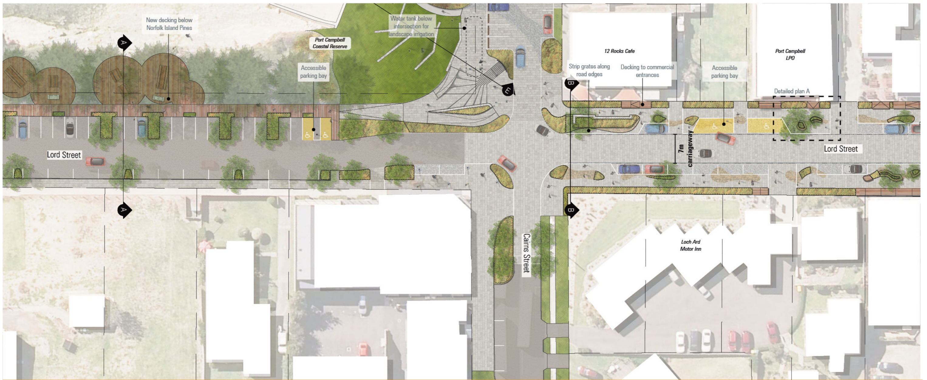
Lord Street Plan - part 2/3 1:500@A3
